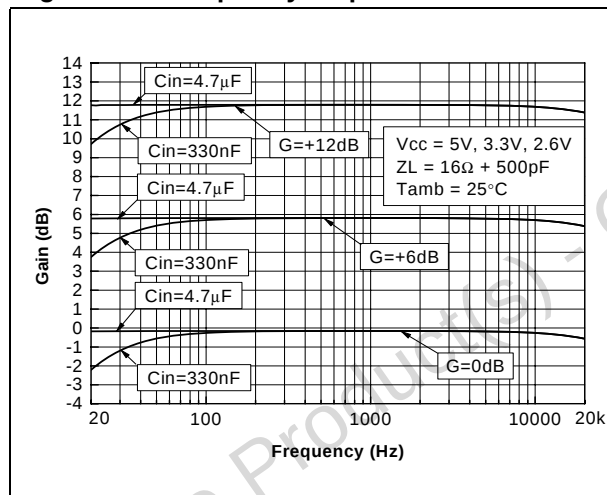
Figure 34. Frequency response
