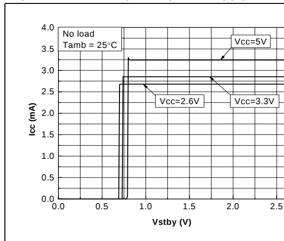
Figure 32. Standby voltage vs. supply current
